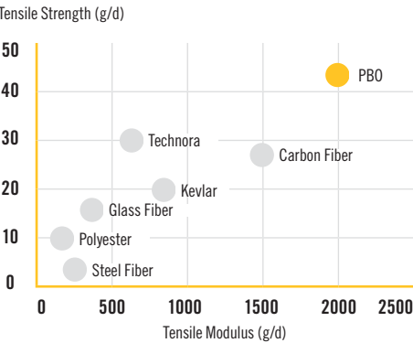
MODULUS & TENSILE STRENGTH (Based on BRP Dynamometer Testing)
